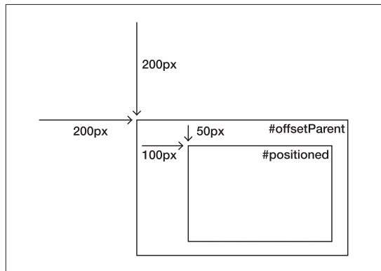
Figure 10.3 How offsetLeft and offsetTop work.
